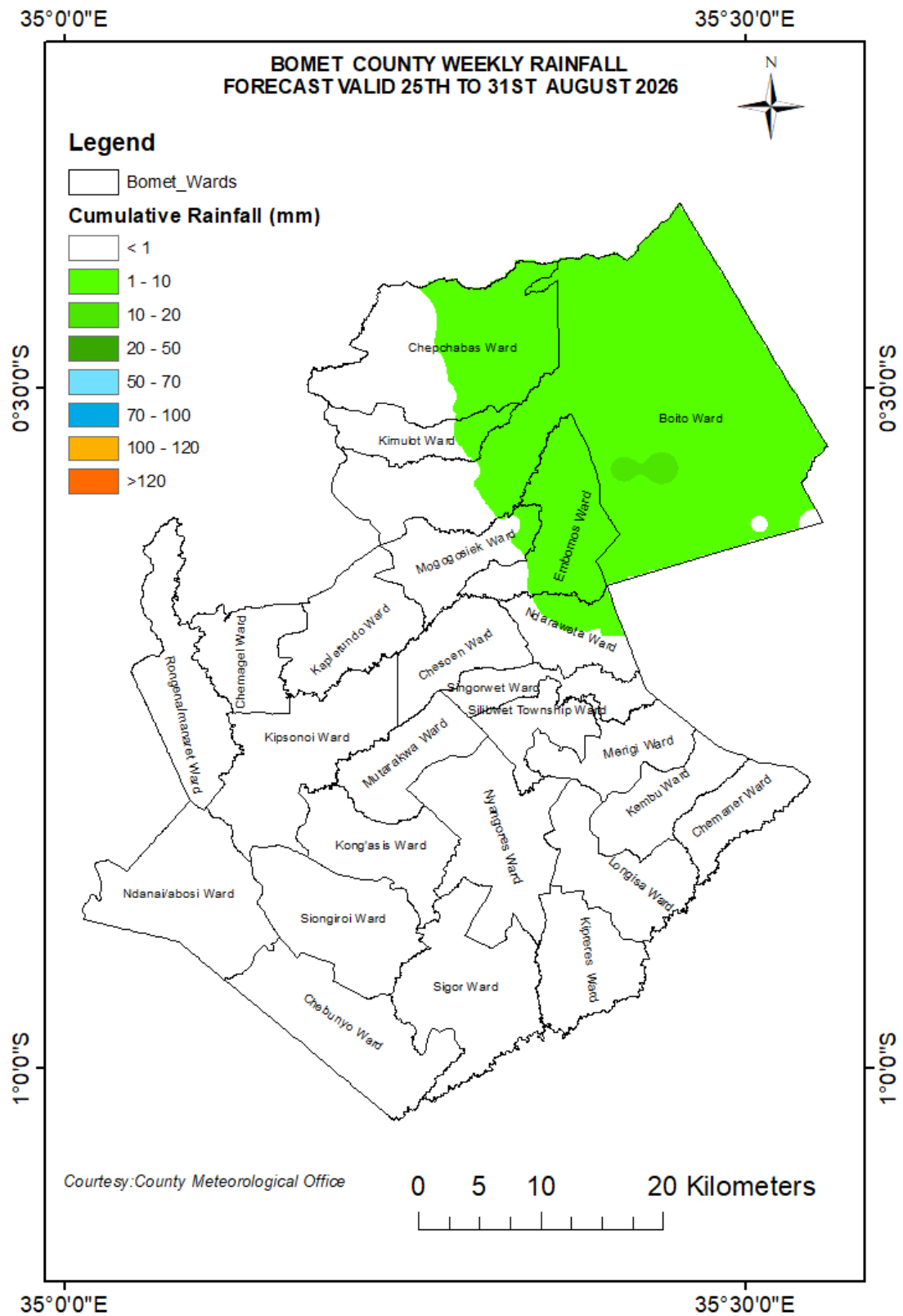
Figure 1: Forecasted Seven-Day Rainfall for 25 th to 31 st August, 2026.
