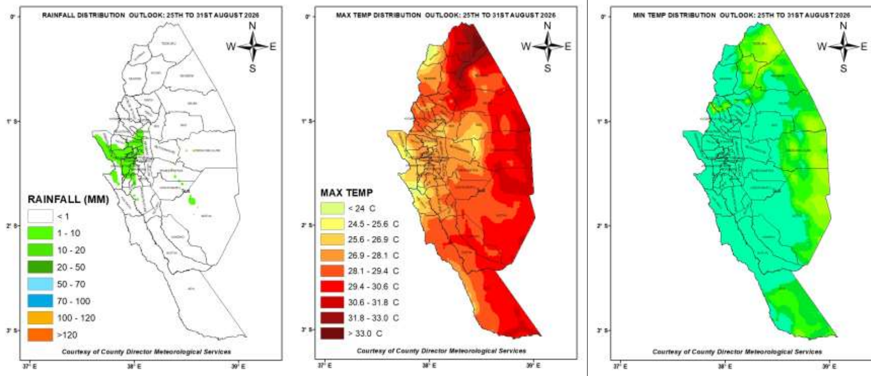
Figure 1: Forecasted Seven-Day Total Rainfall for 25 th to 31 st August 2026
