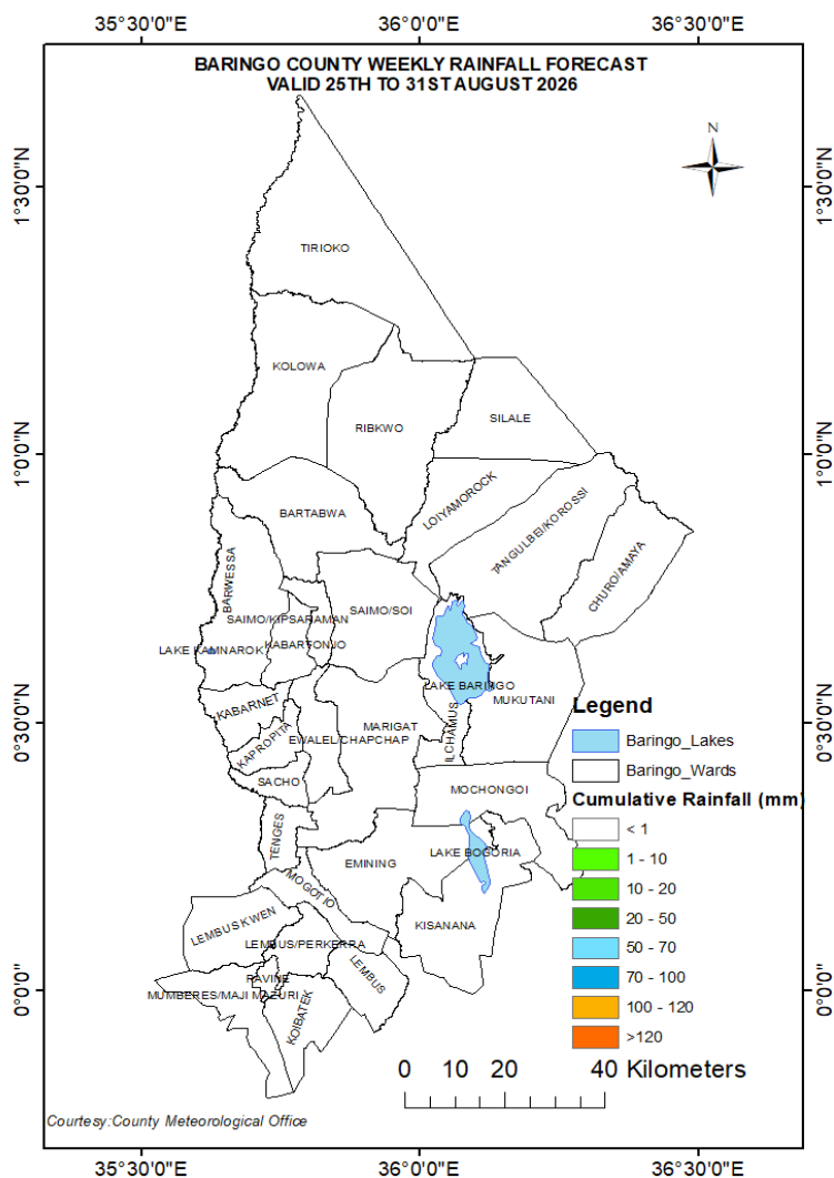
Fig 1. Forecasted cumulative rainfall amounts (mm)
