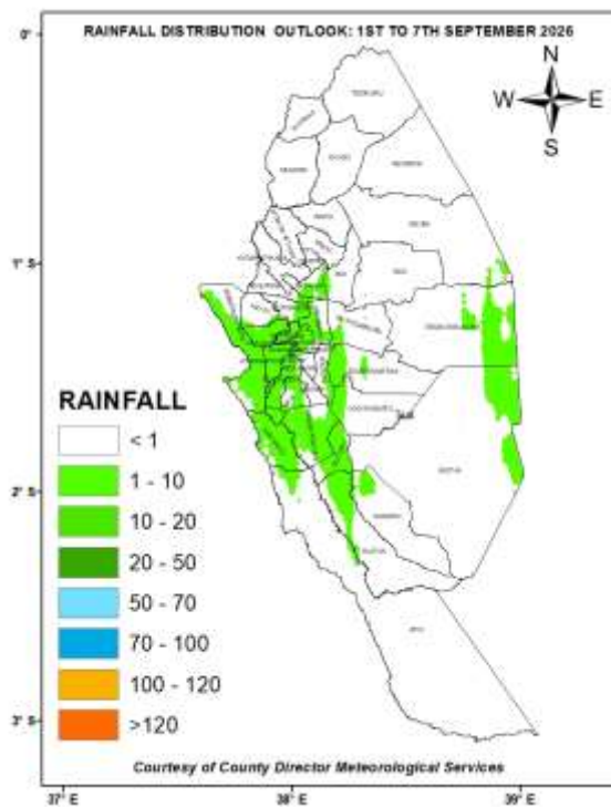
Figure 1: Forecasted Seven-Day Total Rainfall for 1 st to 7 th September 2026
