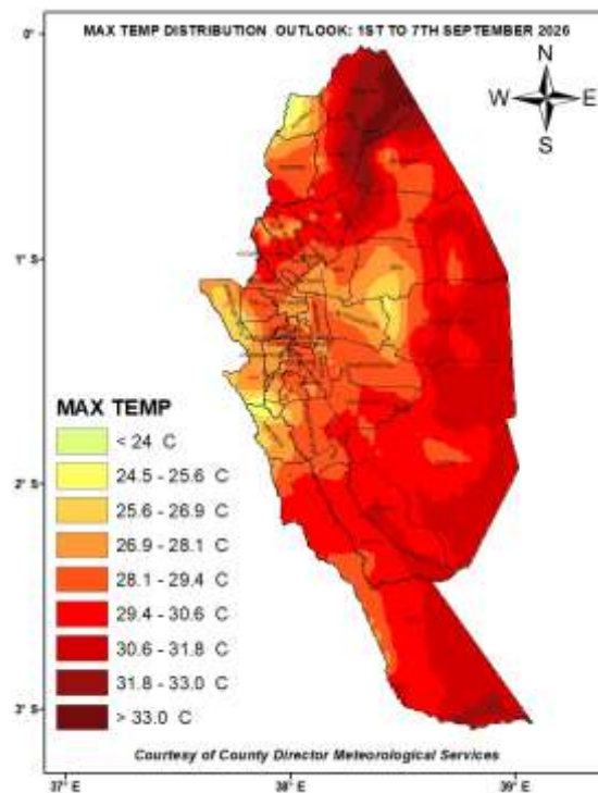
Figure 2: Forecasted Seven-Day Mean Max Temperatures for 1 st to 7 th September 2026
