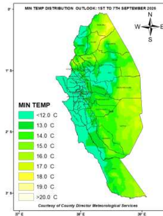
Figure 3: Forecasted Seven-Day Mean Mini Temperatures for 1 st to 7 th September 2026
