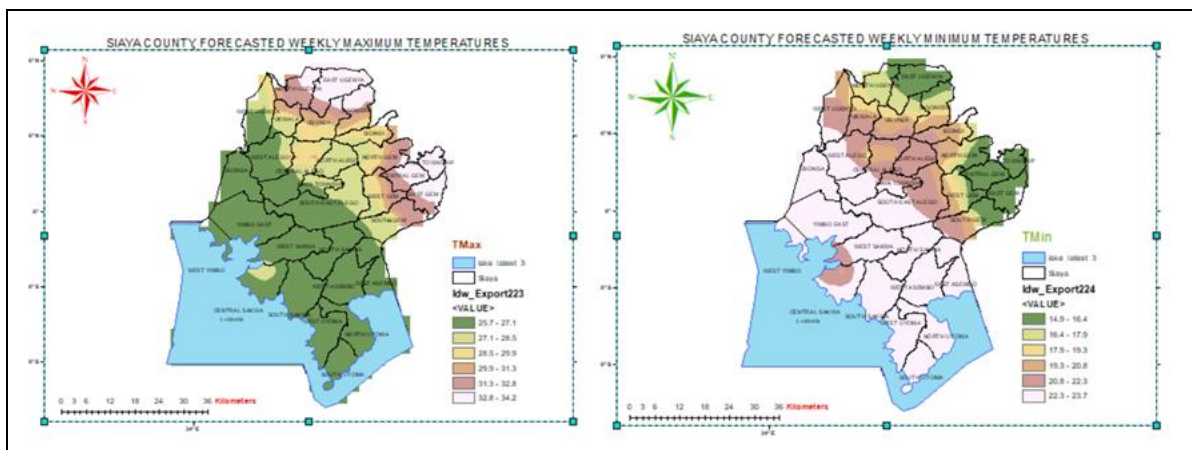
Figure 3a: Forecasted weekly Maximum temperatures
