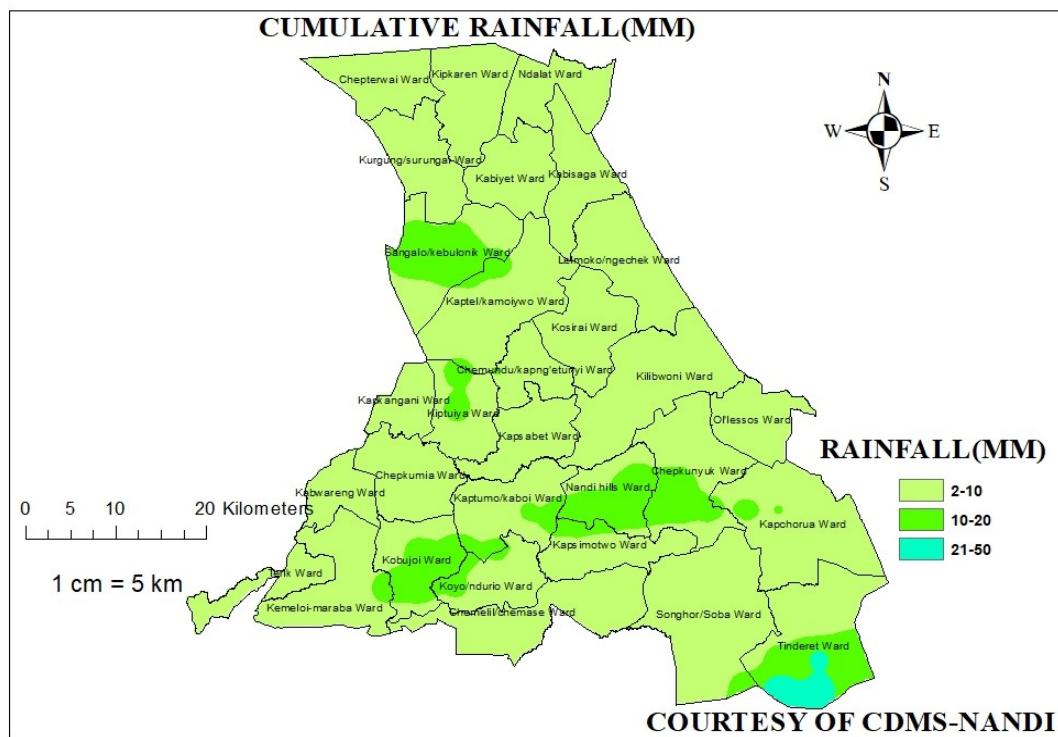
Figure 1: Cumulative rainfall forecast over Nandi County valid 8 th -14 TH Sept 2026
