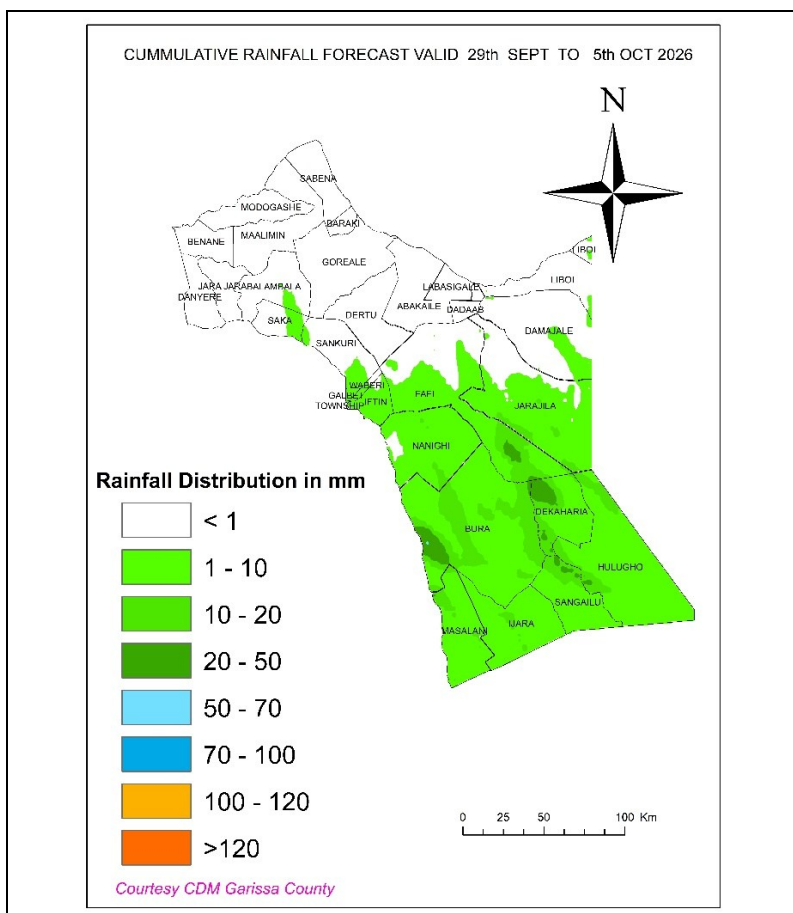
Figure 1: Expected Rainfall distribution over Garissa County valid Tuesday 29 th to Monday 5 th October 2026
