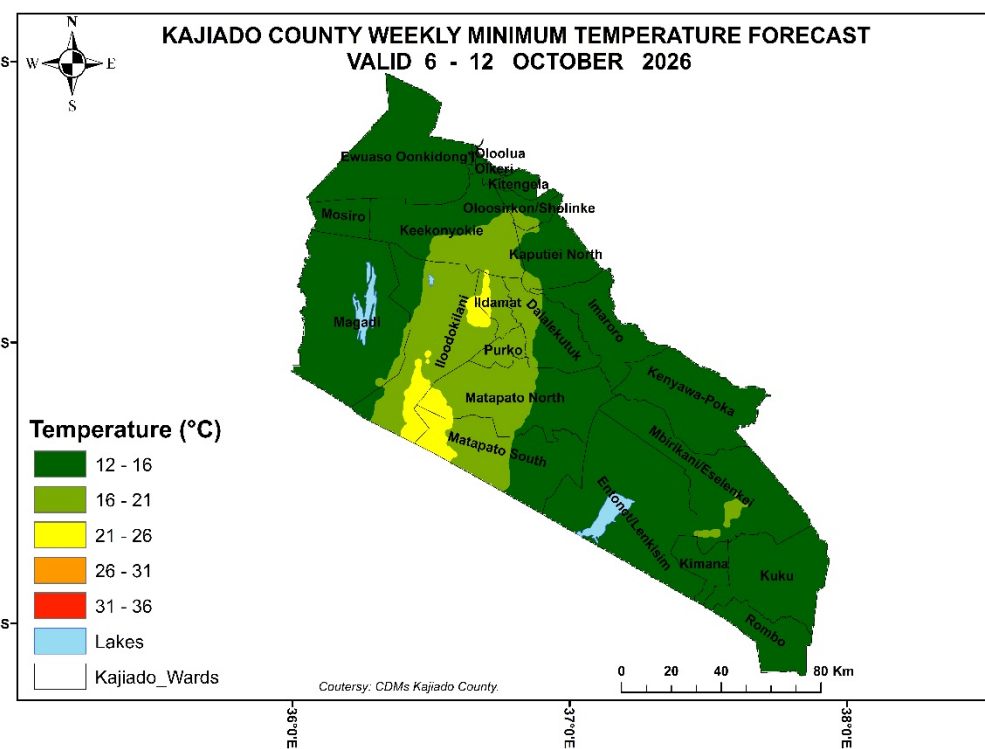
28 Figure 2: Fore casted average Maximum Temperatures for 6 - 12 Oct 2026 Figure 3: Forecasted average Minimum Temperatures for 6 - 12 Oct 2026
