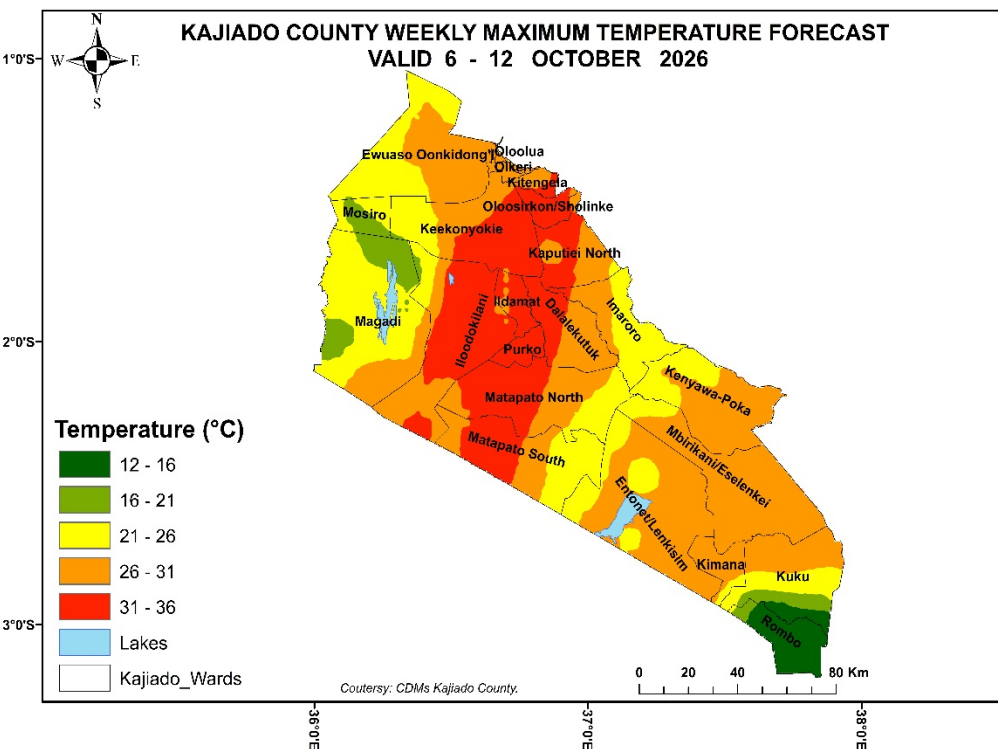
28 Figure 2: Fore casted average Maximum Temperatures for 6 - 12 Oct 2026 Figure 3: Forecasted average Minimum Temperatures for 6 - 12 Oct 2026
