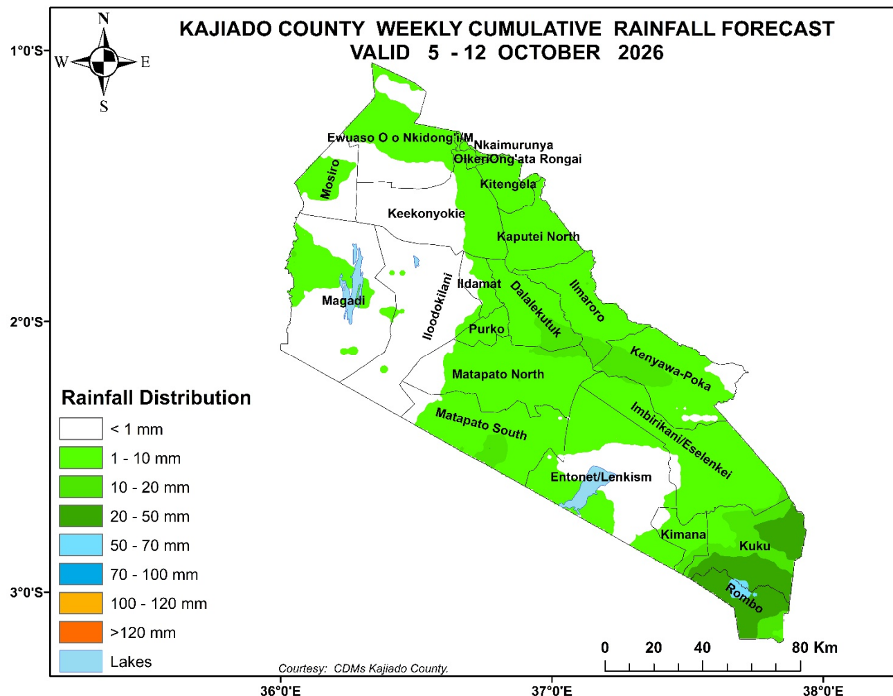
Figure 1: Forecasted seven-day total rainfall for 6 - 12 Oct 2026
