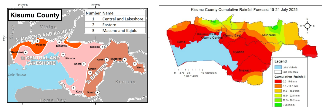
Figure 1: Climatic zones (left) Cumulative rainfall forecast (right)
