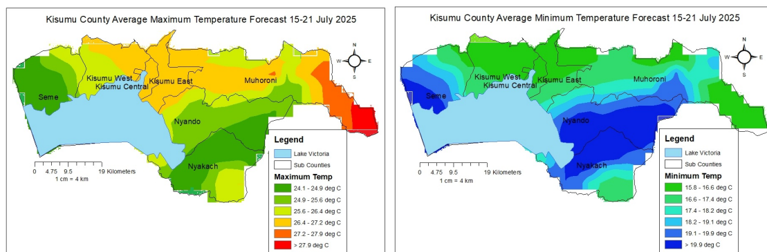
Figure 2: Average maximum (left) and minimum (right) temperature forecast
