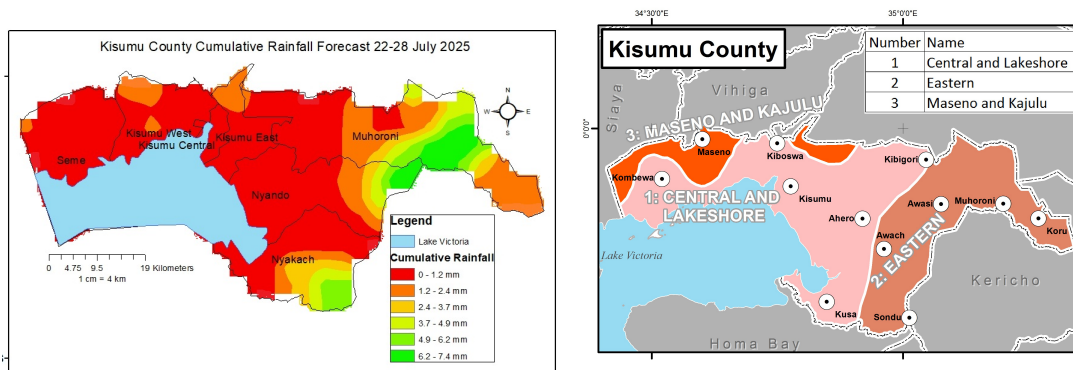
Figure 1: Cumulative rainfall forecast (left) Climatic zones (right)
