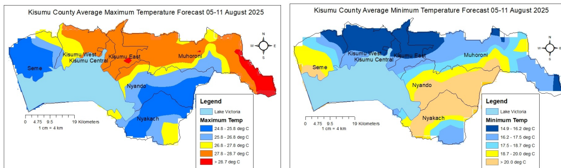
Figure 2: Average maximum (left) and minimum (right) temperature forecast
