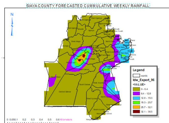
Figure 2: Forecasted cumulative weekly rainfall from 5 th to 11 th August 2025
