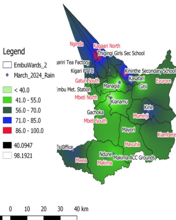
Rainfall Performance in March 2024 Over Embu County
