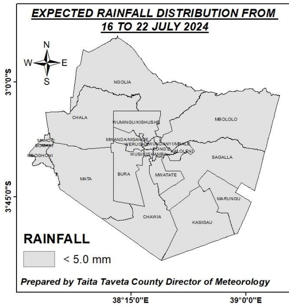
Figure 1 Expected Rainfall Distribution from 16 to 22 July 2024
