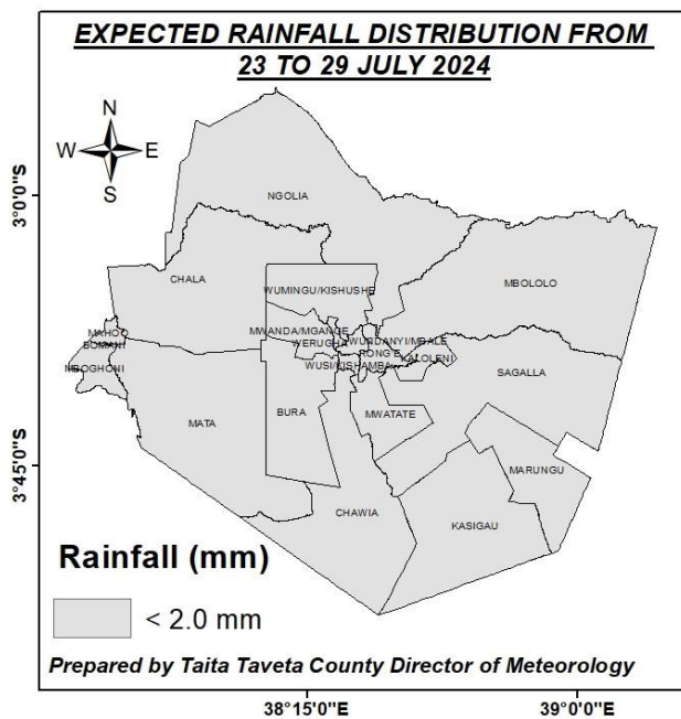
Figure 1 Expected Rainfall Distribution from 23 to 29 July 2024
