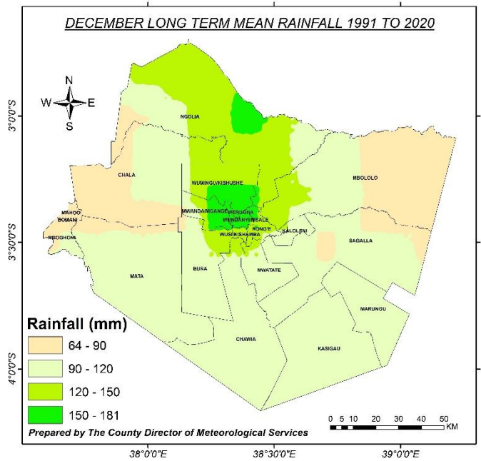
Figure 1: December Long Term Mean Rainfall 1991 to 2020
