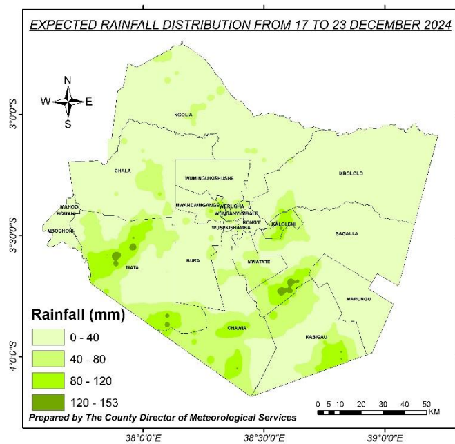
Figure 2 : Expected Rainfall Distribution from 17th to 23rd Dec..
