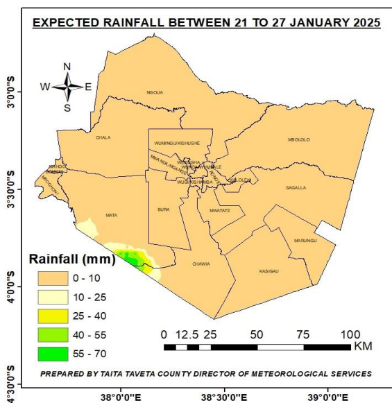
Figure 1 : Expected Rainfall from 21 to 27 January 2025
