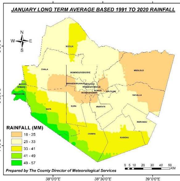
Figure 2: January Long Term Average Rainfall 1991 to 2020
