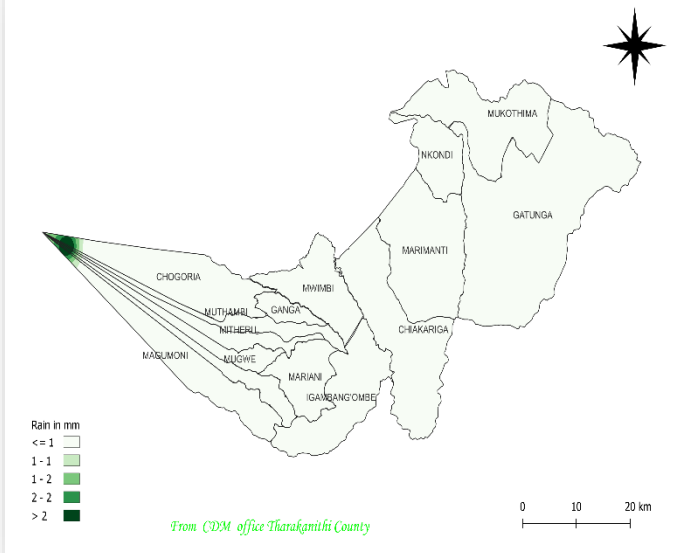
Tharakanithi weather outlook valid 4th -10th Feb 2025
