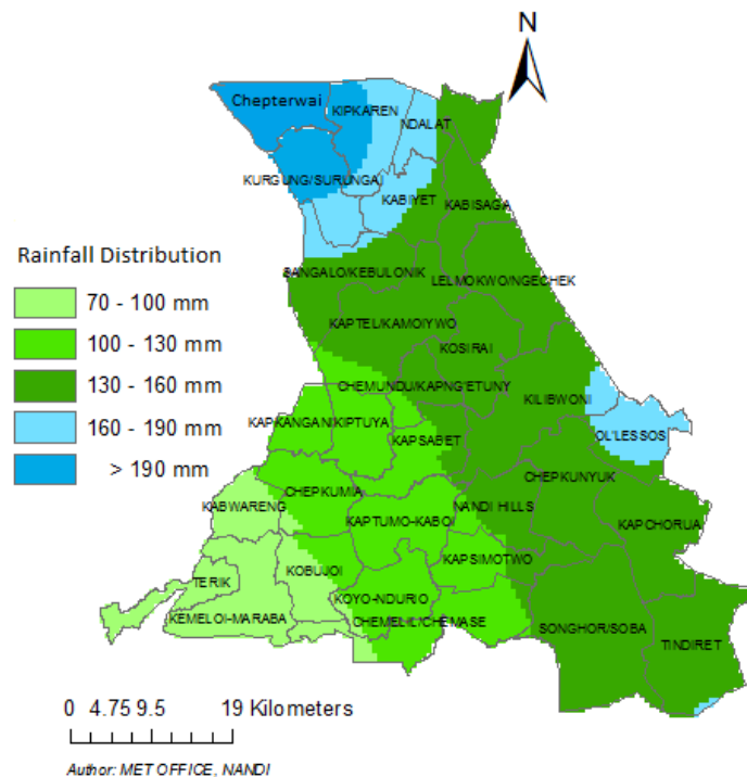
Figure 1: Forecasted Seven-Day total rainfall valid 15 th to 21 st April 2025
