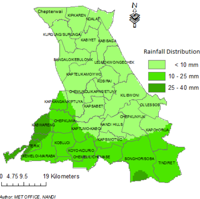
Figure 1: Forecasted Seven-Day total rainfall valid 22 nd to 28 th April 2025
