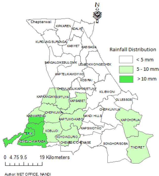
Figure 1: Forecasted Seven-Day total rainfall valid 1 st to 7 th April 2025
