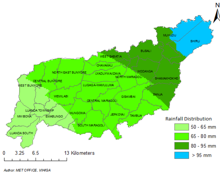
Figure 1: Forecasted Seven-Day total rainfall valid 15 th to 21 st April 2025
