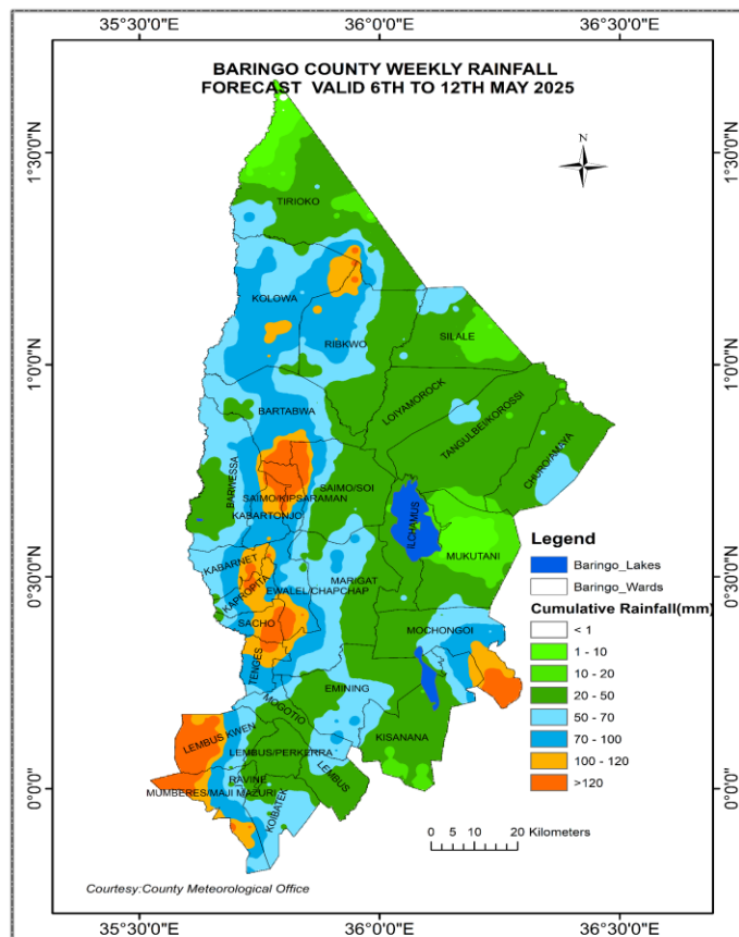
Fig 1. Forecasted cumulative rainfall amounts (mm)
