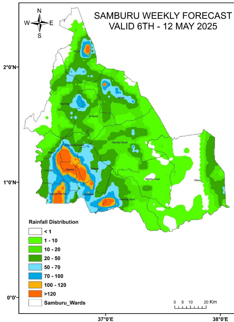
Figure1:Samburu County Cumulative rainfall forecast
